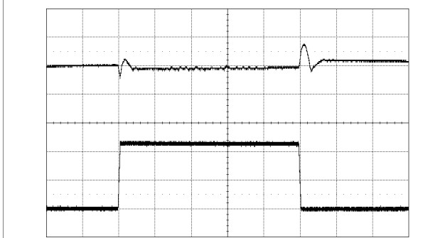
Output voltage response to load current Step-change (6.25-18.75-6.25 A) at: T_{P1} = +25 °C, V_I = 12 V, V_O = 1.0 V di/dt = 2 A/ \mu s, f_{sw} = 320 kHz C_O = 470 \mu F/10 m \Omega Top trace: output voltage (200 mV/div.). Bottom trace: load current (5 A/div.). Time scale: (0.1 ms/div.).
