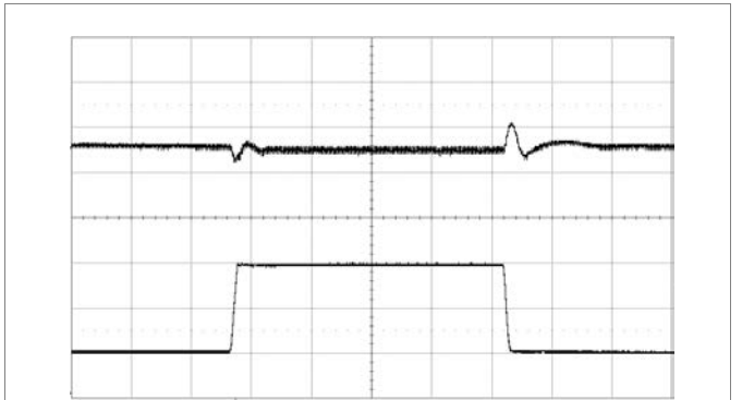
Output voltage response to load current step-change (5-15-5 A) at: T_{P1} = +25 ^{\circ} C, V_I = 12 V, V_O = 1.0 V, di/dt = 2 A/ \mu s, f_{sw} = 320 kHz, C_O = 470 \mu F/10 m \Omega . Top trace: output voltage (200 mV/div.). Bottom trace: load current (5 A/div.). Time scale: (0.1 ms/div.).
