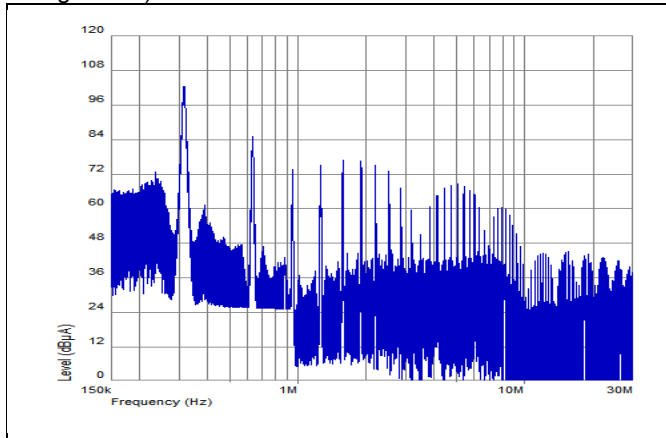
EMI without filter for BMR 463 0008
