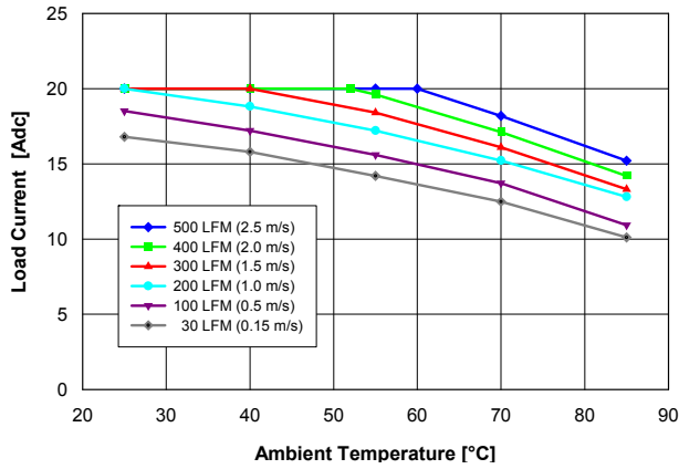
Fig. 1 : Available load current vs. ambient air temperature and airflow rates for converter with G height pins mounted vertically with air flowing from pin 1 to pin 3, MOSFET temperature \leq 125\text{ }^{\circ}\text{C} , V_{in} = 48\text{ V} .
