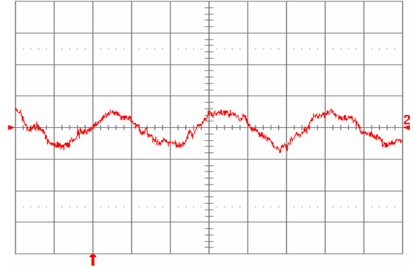
Fig. 14: Input reflected ripple current, i_c (10 mA/div.), measured through 10 \mu H at the source at full rated load current and V_{in} = 48 V. Refer to Fig. 12 for test setup. Time scale: 1 \mu s/div.
