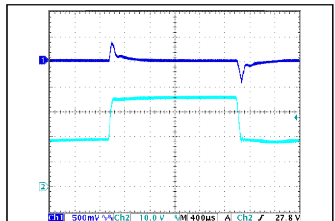
Figure 6: Output voltage response to step-change in input voltage (300 V/ms). Load cap: 100 \mu\text{F} , electrolytic output capacitance. Ch 1: V out (500 mV/div), Ch 2: V in (10 V/div).
