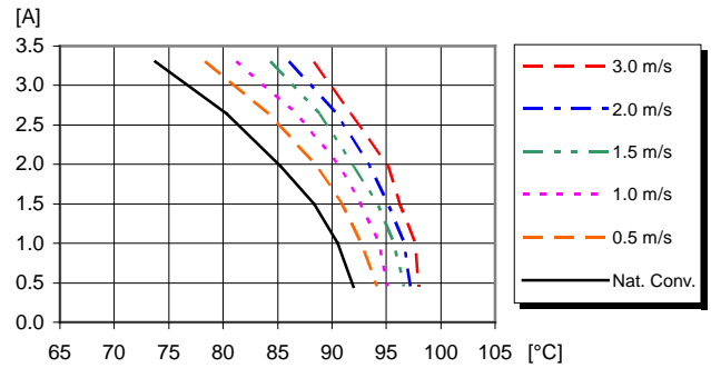
Available load current vs. ambient air temperature and airflow at V_i = 48\text{ V} , V_o = 30\text{ V} . See Thermal Consideration section.
