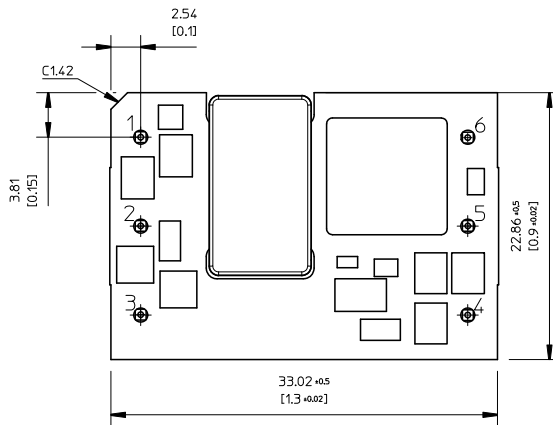
RECOMMENDED FOOTPRINT - TOP VIEW
