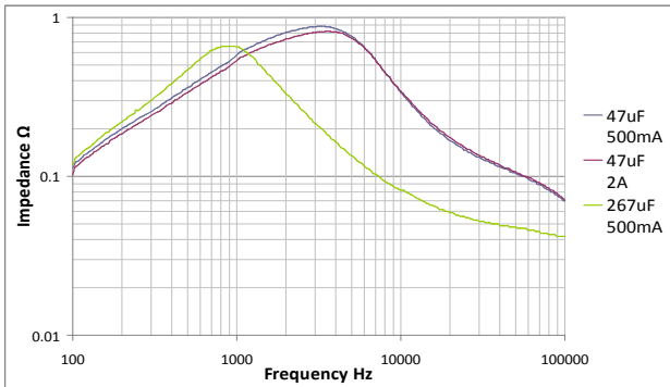
Output Impedance vs. frequency at V_i = 48\text{ V} , V_o = 30\text{ V} .
