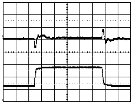
Output voltage response to load current step- change (30-60-30 A) at: T_{ref} = +25^\circ\text{C} , V_I = 3.3 V. Top trace: output voltage (100 mV/div.). Bottom trace: load current (20 A/div.). Time scale: 0.1 ms/div.
