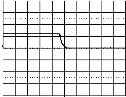
Shut-down enabled by disconnecting V_I at: T_{ref} = +25^\circ\text{C} , I_O = 60 A resistive load, V_I = 3.3 V. Top trace: output voltage (1.0 V/div.). Time scale: 1.0 ms/div.
