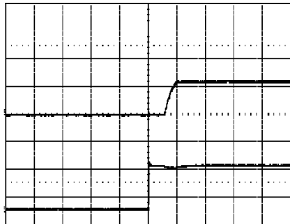
Start-up enabled by connecting V_I at: T_{ref} = +25^\circ\text{C} , I_O = 60 A resistive load, V_I = 3.3 V. Top trace: output voltage (1.0 V/div.). Bottom trace: input voltage (2.0 V/div.). Time scale: 10 ms/div.
